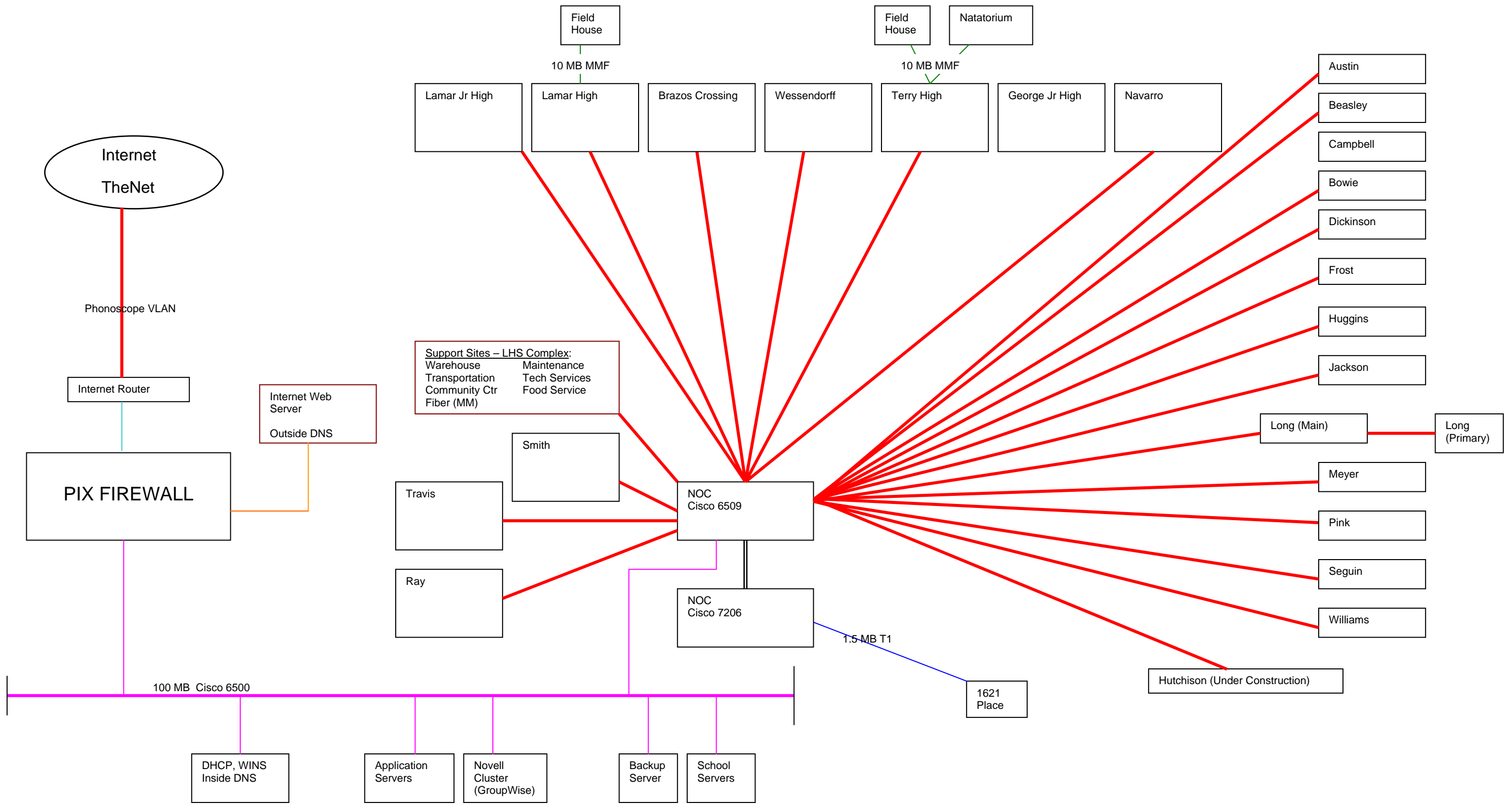
Lamar Consolidated Independent School District Wide Area Network Diagram 12/6/2004
